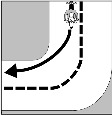
Constant curves
