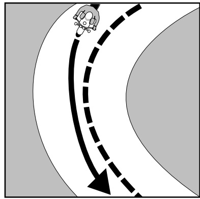
Widening curves
