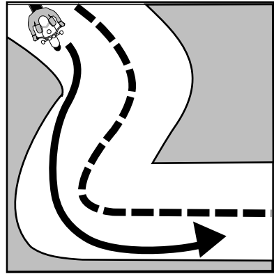
Multiple curves
